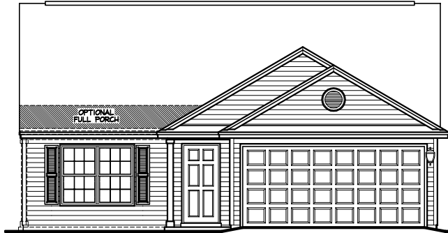
VINYL FRONT ELEVATION
