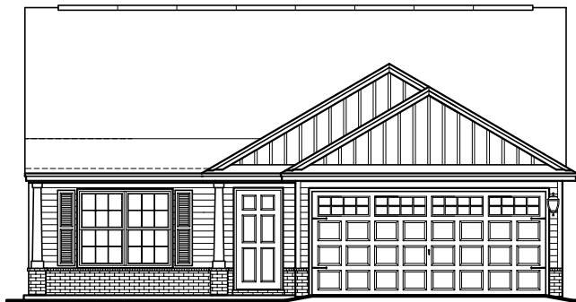
CARRIAGE FRONT ELEVATION
